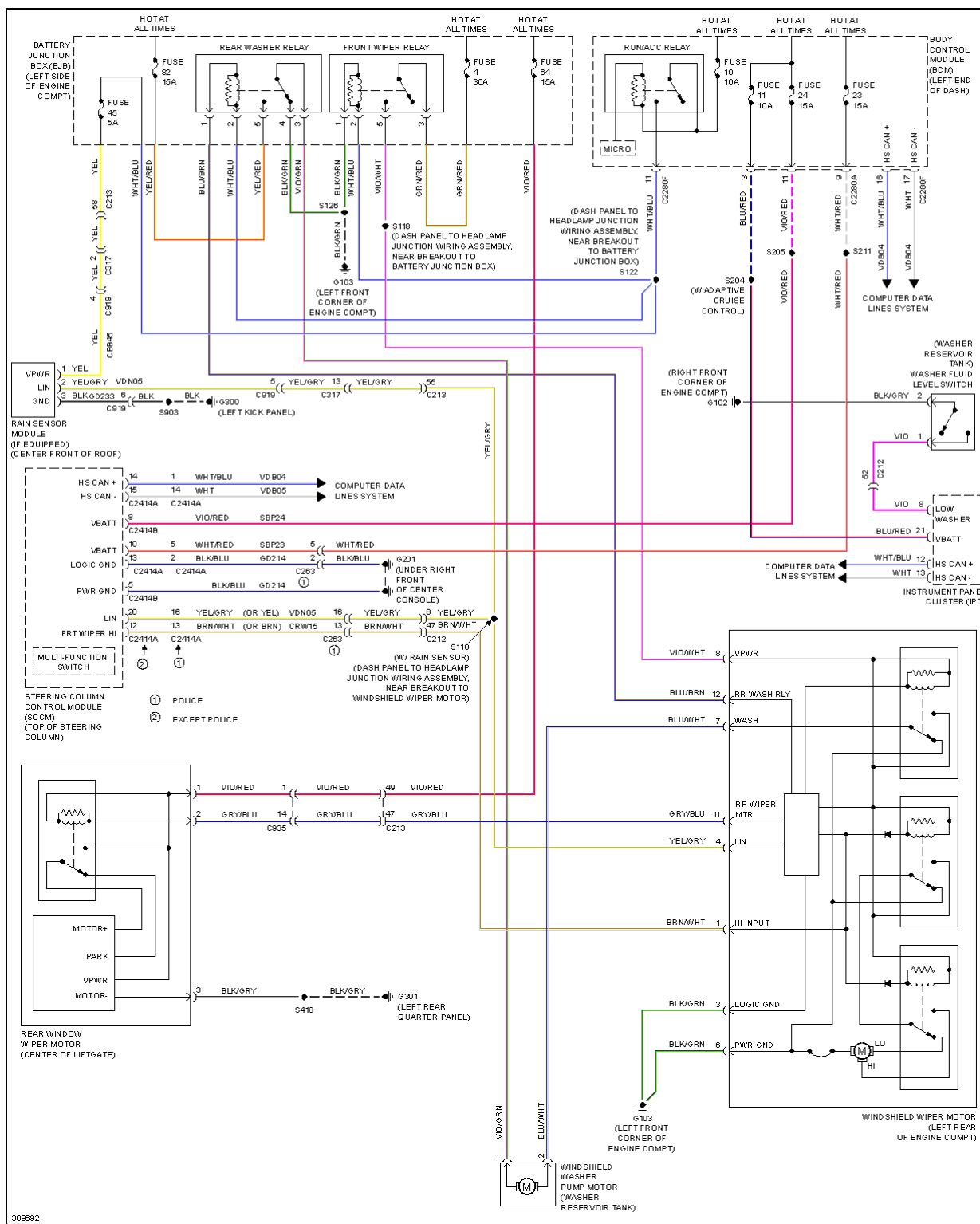
Fig. 132: Wiper/Washer Circuit
