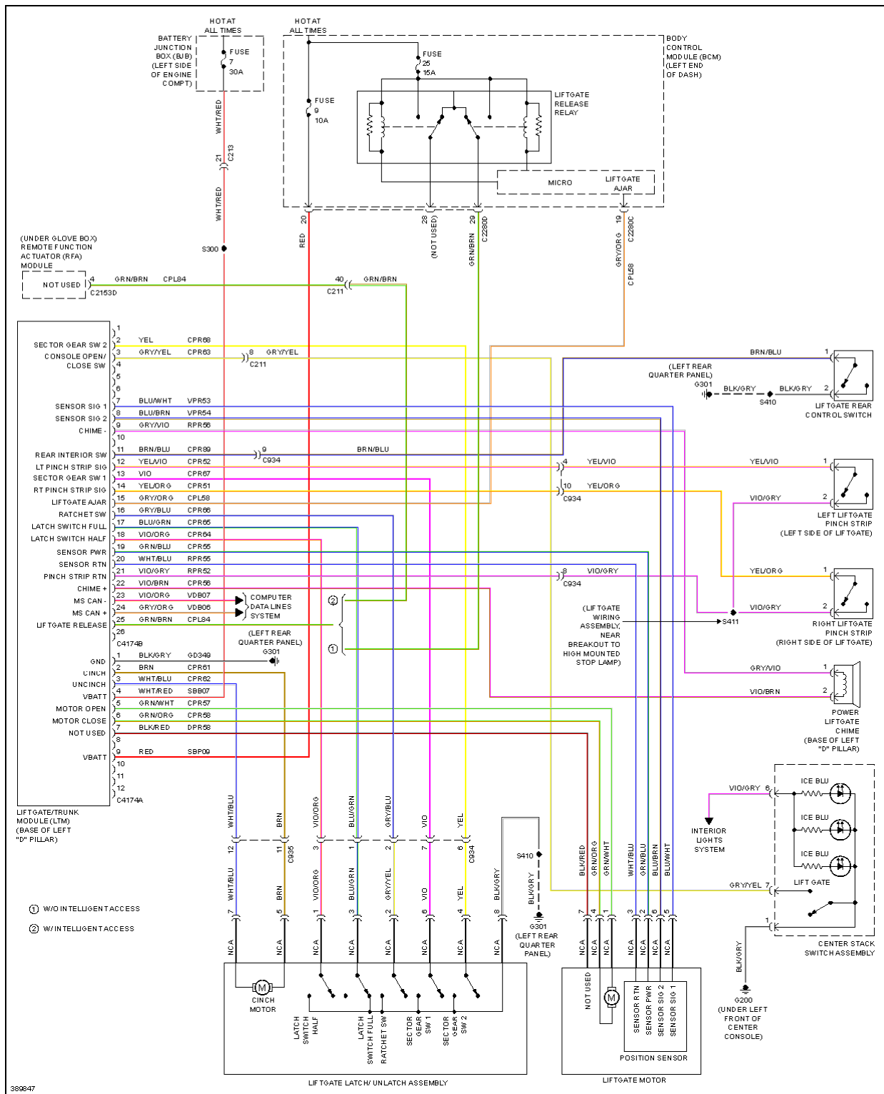
Fig. 129: Power Liftgate Circuit
