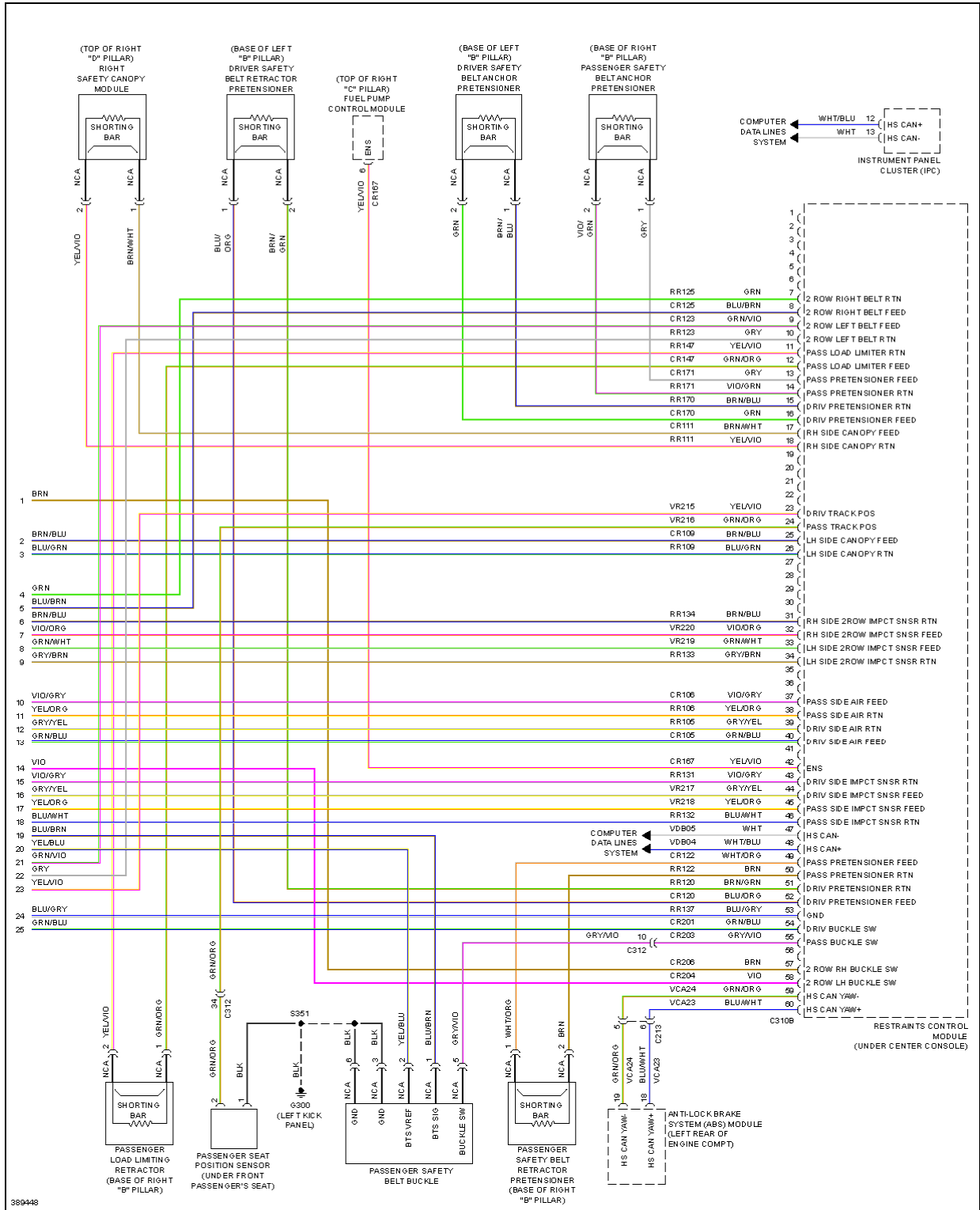
Fig. 119: Supplemental Restraints Circuit (3 of 3)
