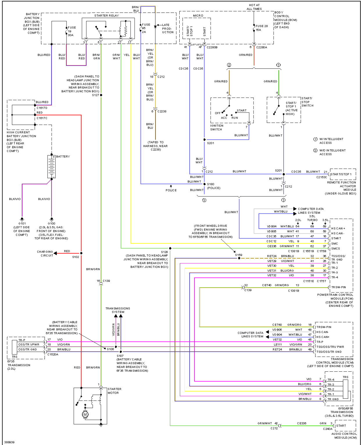
Fig. 116: Starting Circuit
