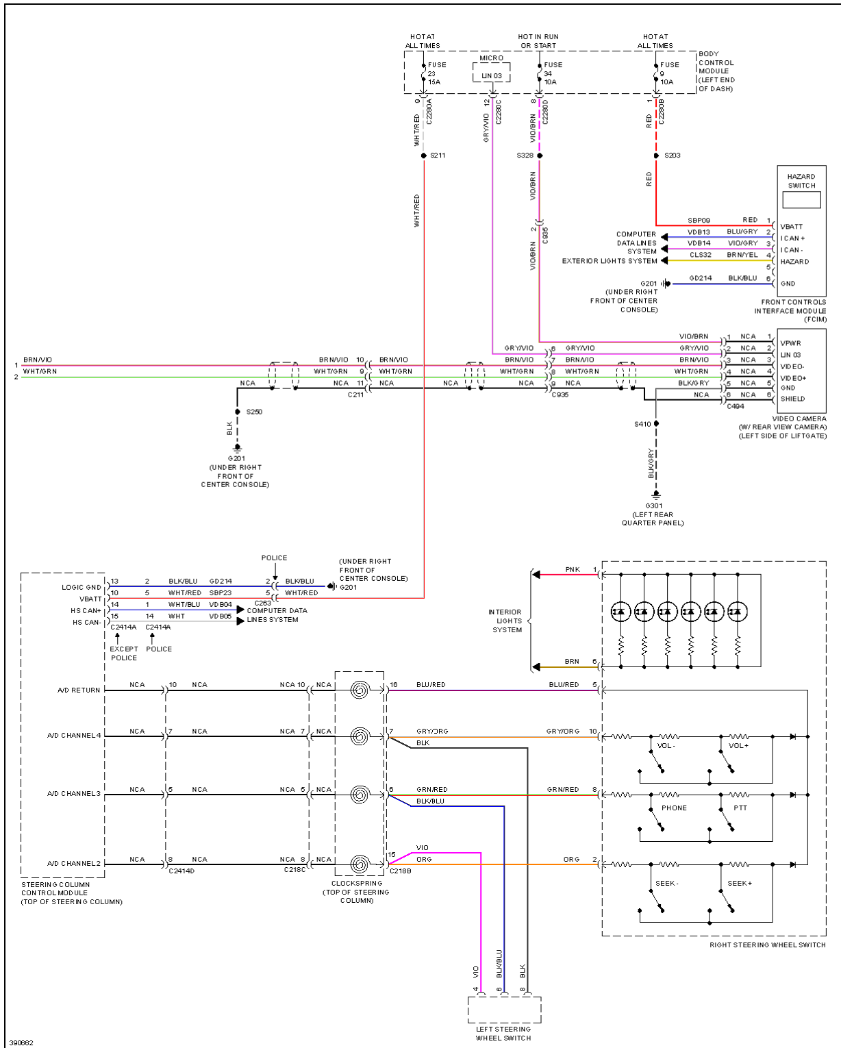
Fig. 112: SYNC Radio Circuit, W/ SYNC GEN 2 (2 of 2)
