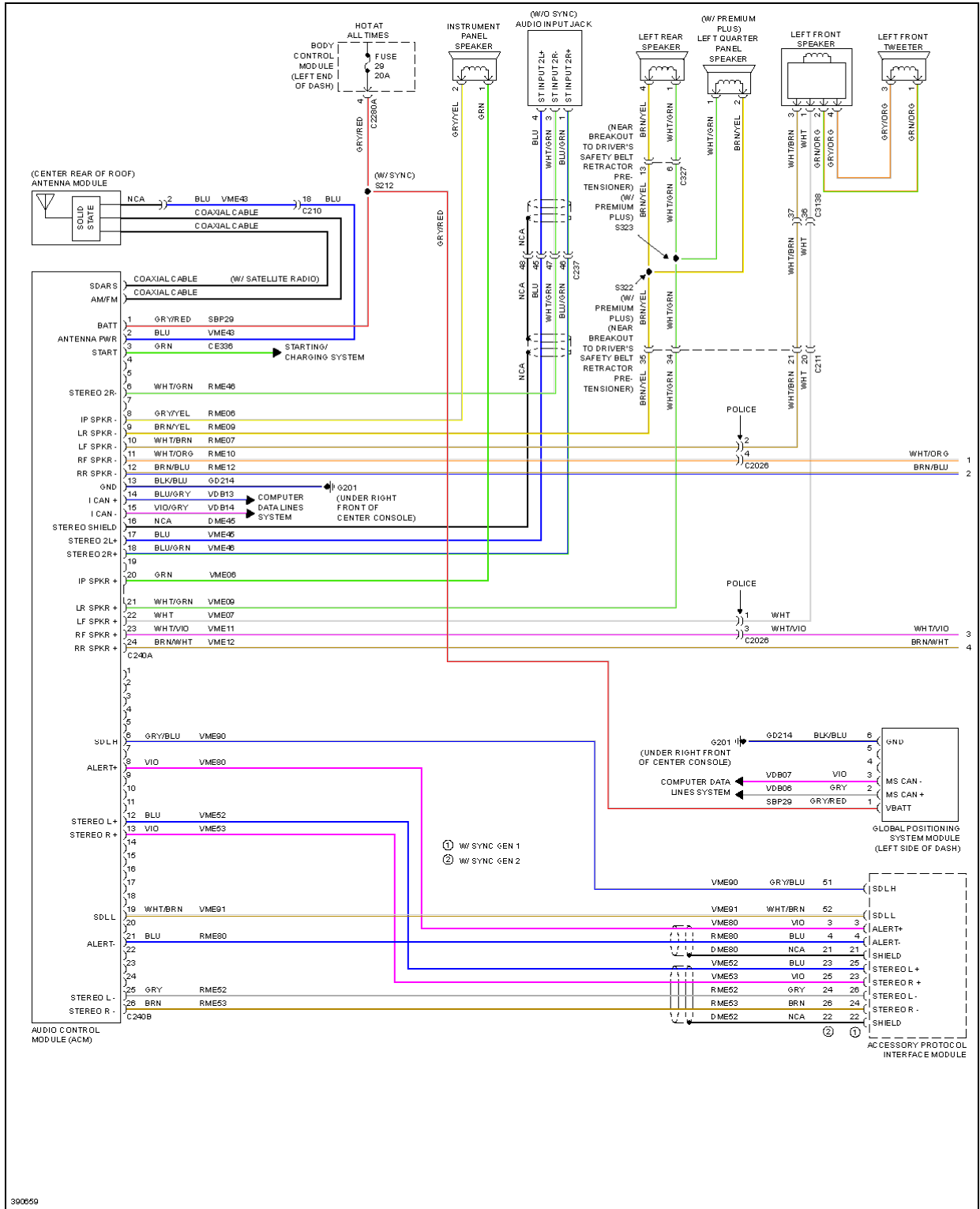
Fig. 105: Premium Radio Circuit (1 of 2)
