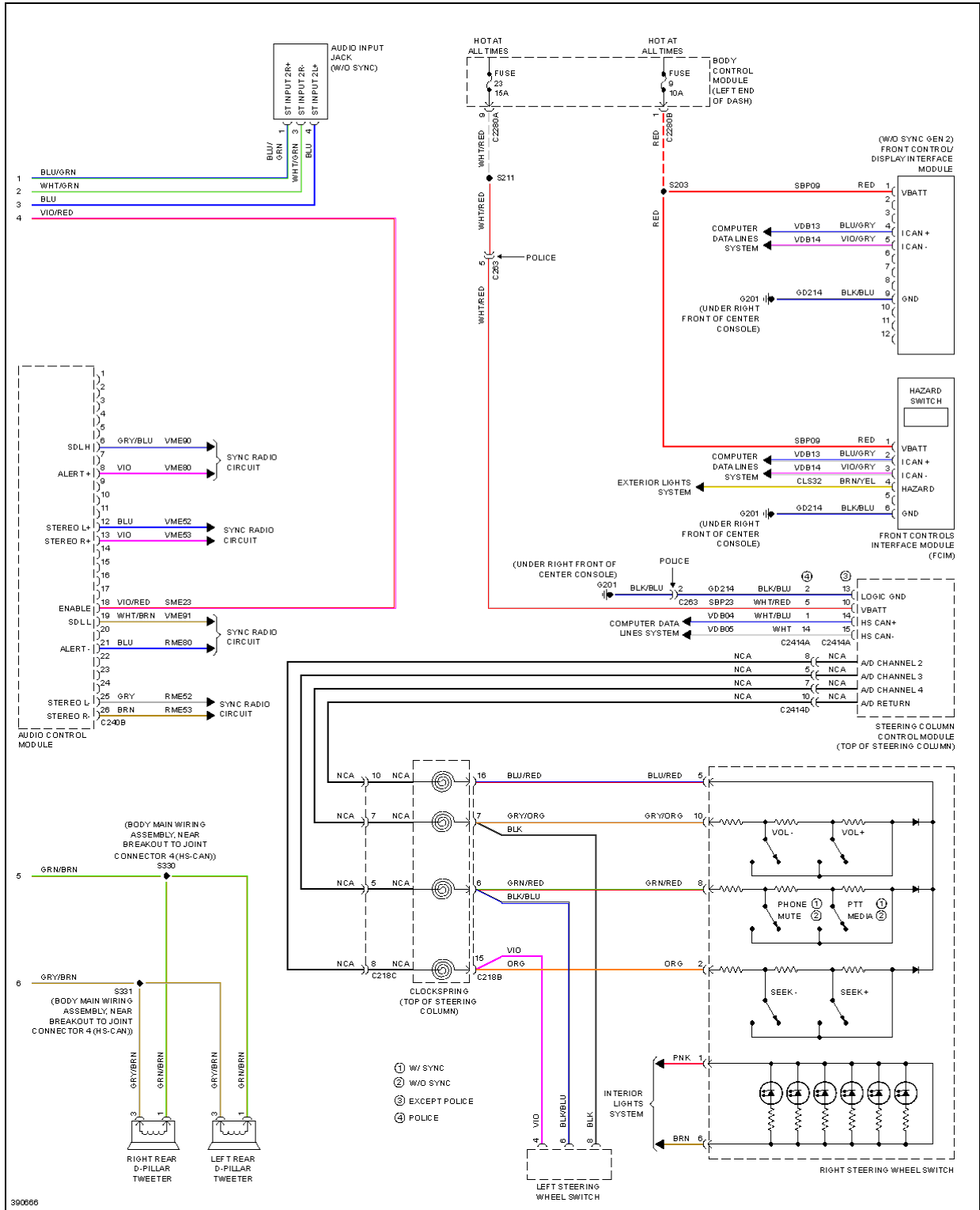
Fig. 108: SONY Radio Circuit (2 of 2)
