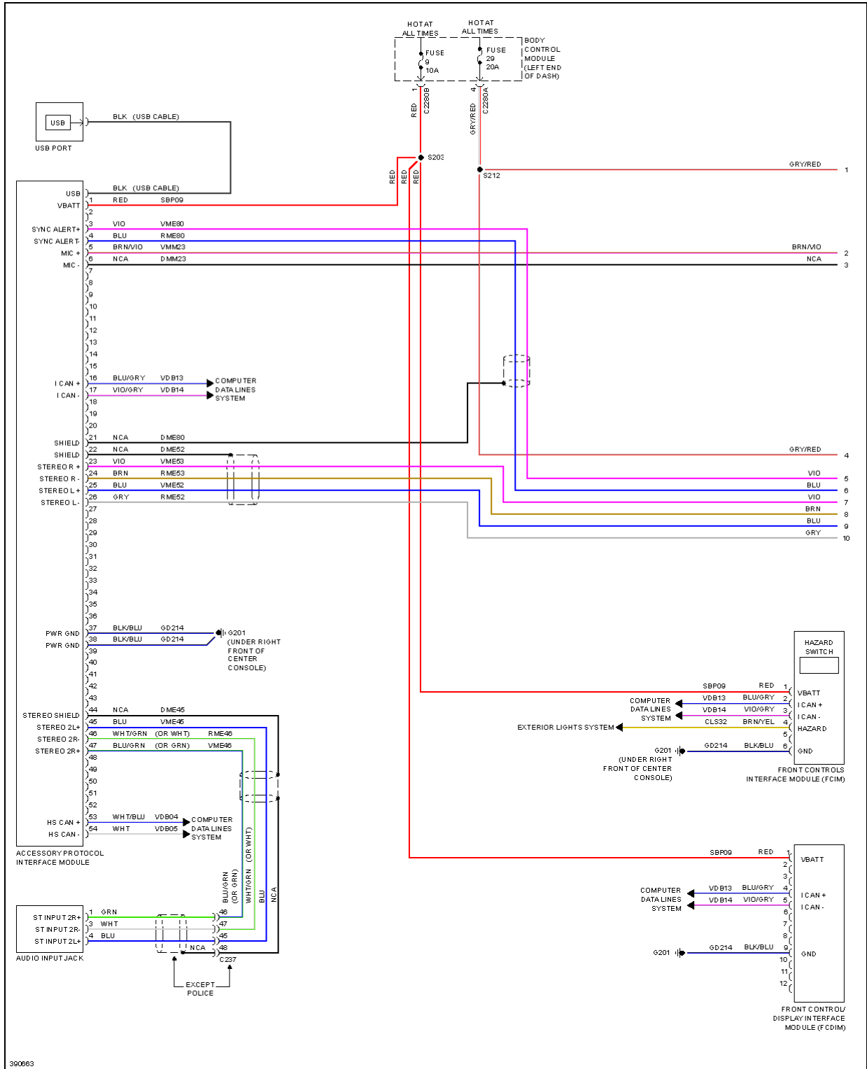
Fig. 109: SYNC Radio Circuit, W/ SYNC GEN 1 (1 of 2)
