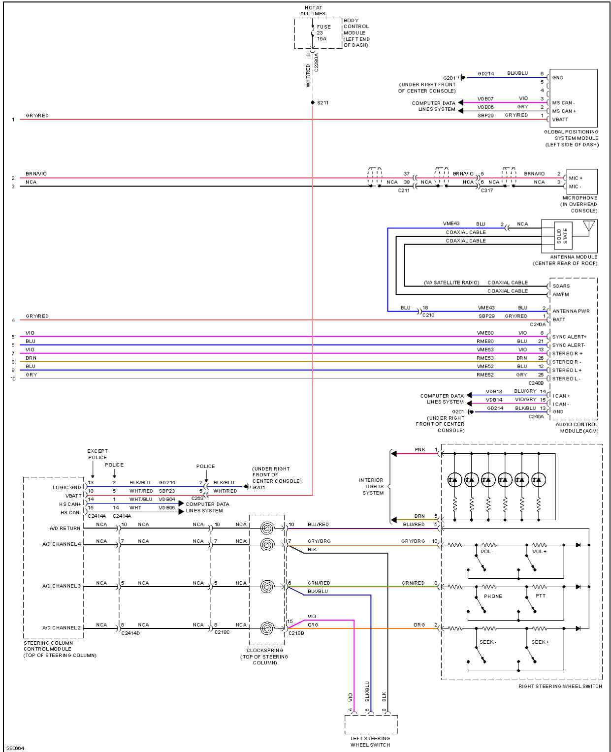
Fig. 110: SYNC Radio Circuit, W/ SYNC GEN 1 (2 of 2)
