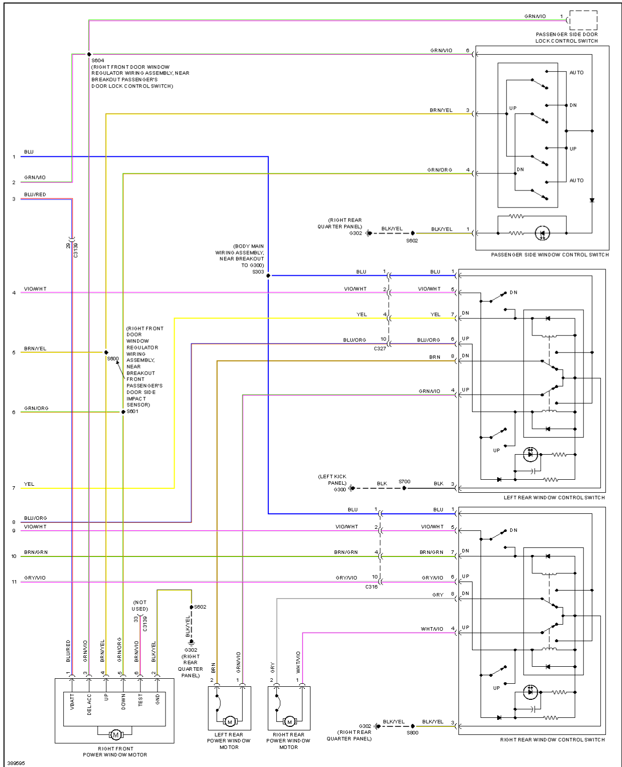
Fig. 104: Power Windows Circuit, XLT, Limited & Sport (2 of 2)
