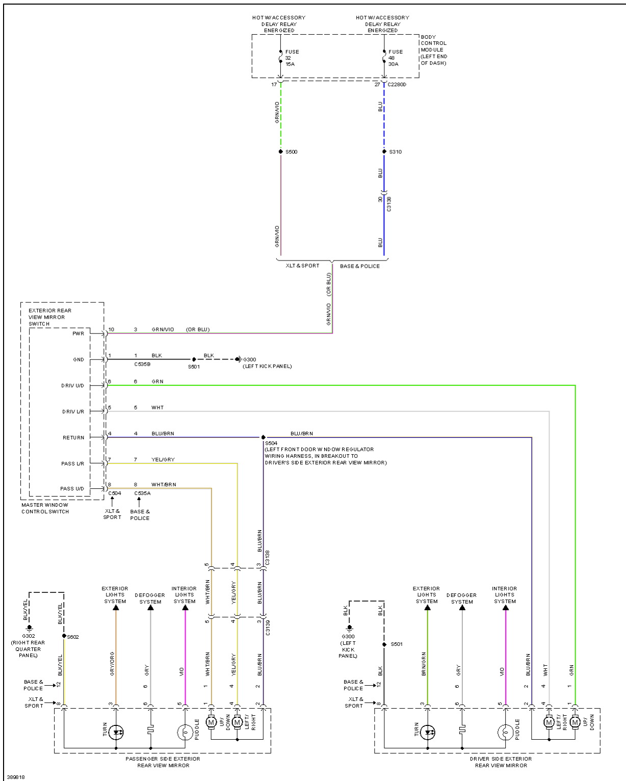
Fig. 88: Power Mirrors Circuit
