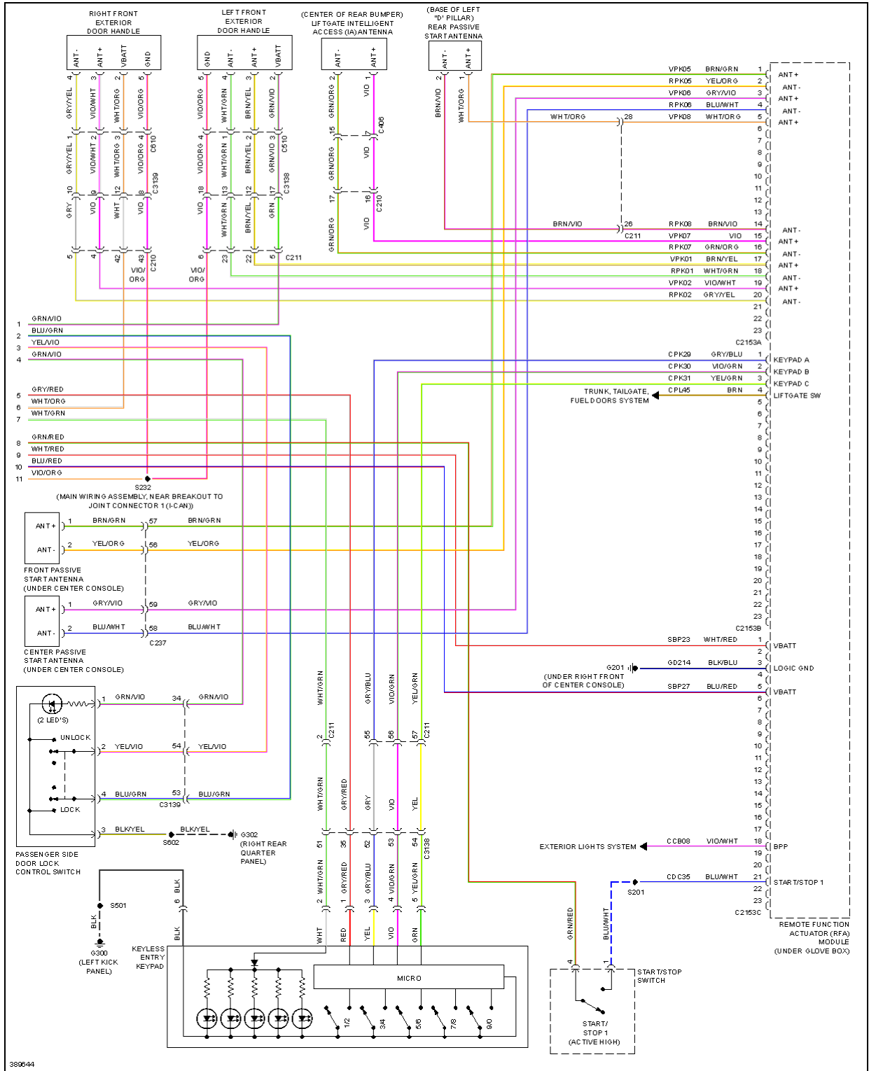
Fig. 83: Power Door Locks Circuit, W/ Intelligent Access (2 of 2)
