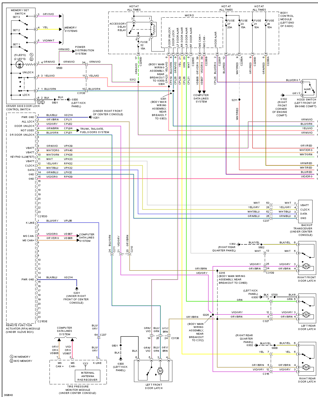
Fig. 82: Power Door Locks Circuit, W/ Intelligent Access (1 of 2)
