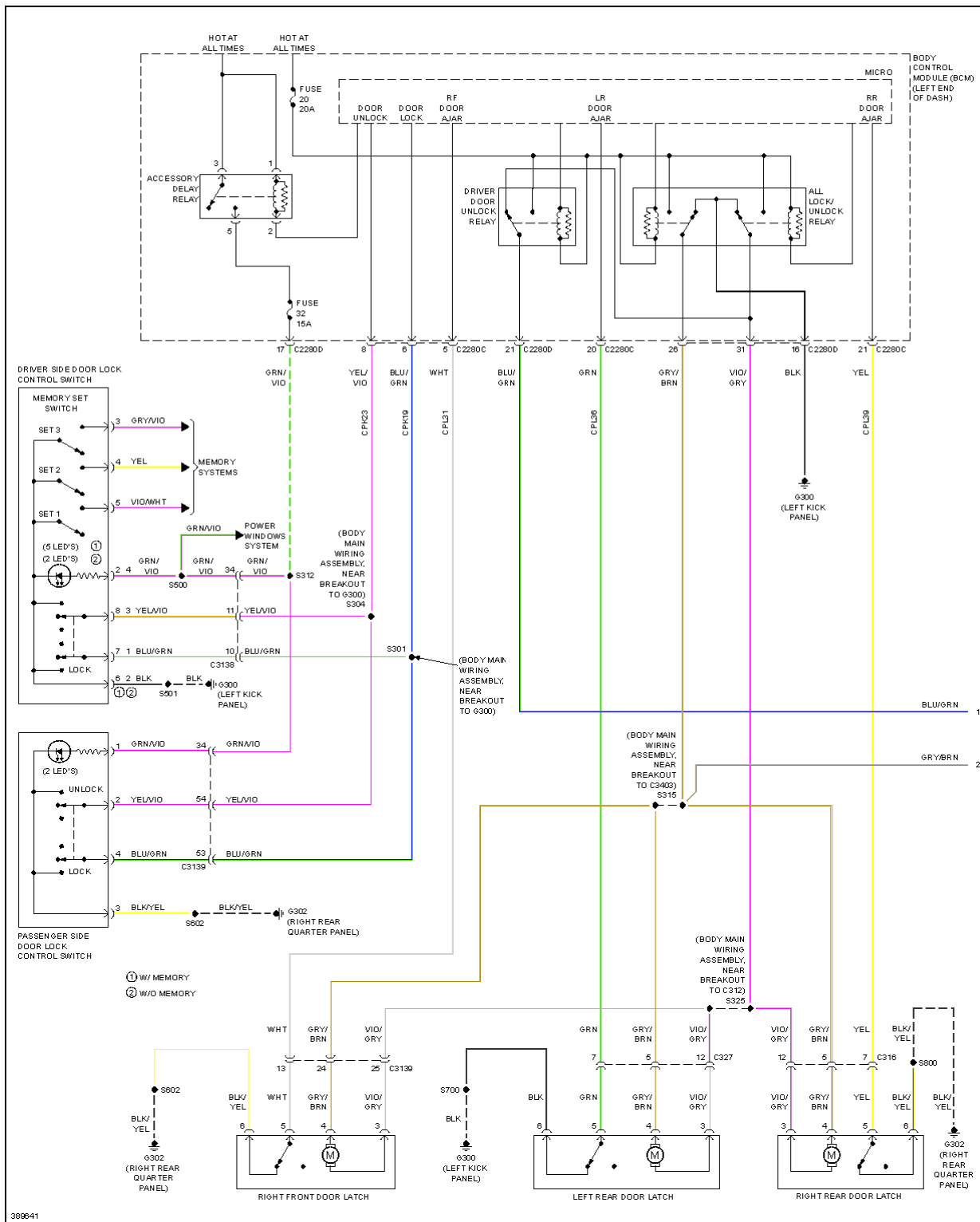
Fig. 84: Power Door Locks Circuit, W/O Intelligent Access (1 of 2)
