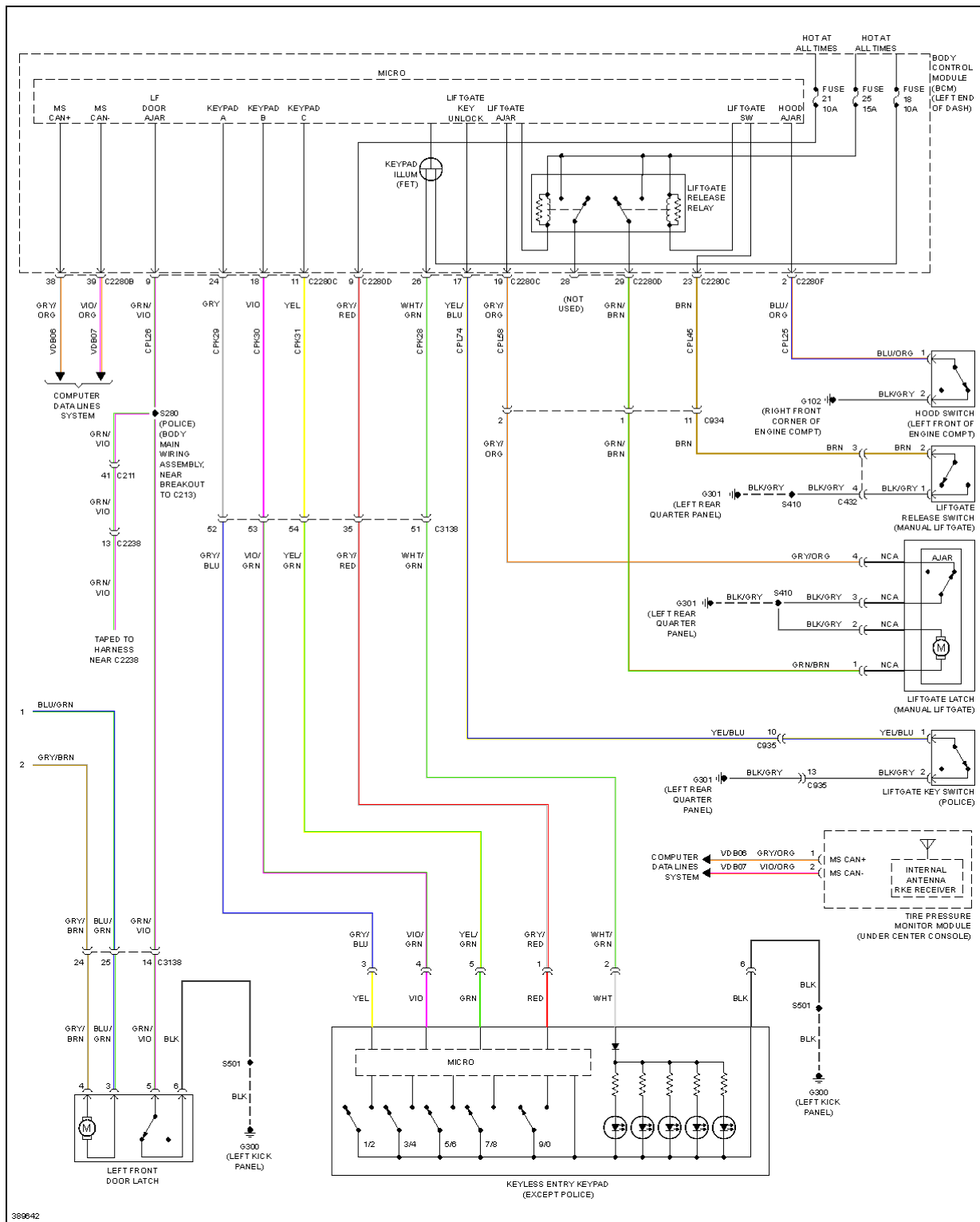
Fig. 85: Power Door Locks Circuit, W/O Intelligent Access (2 of 2)
