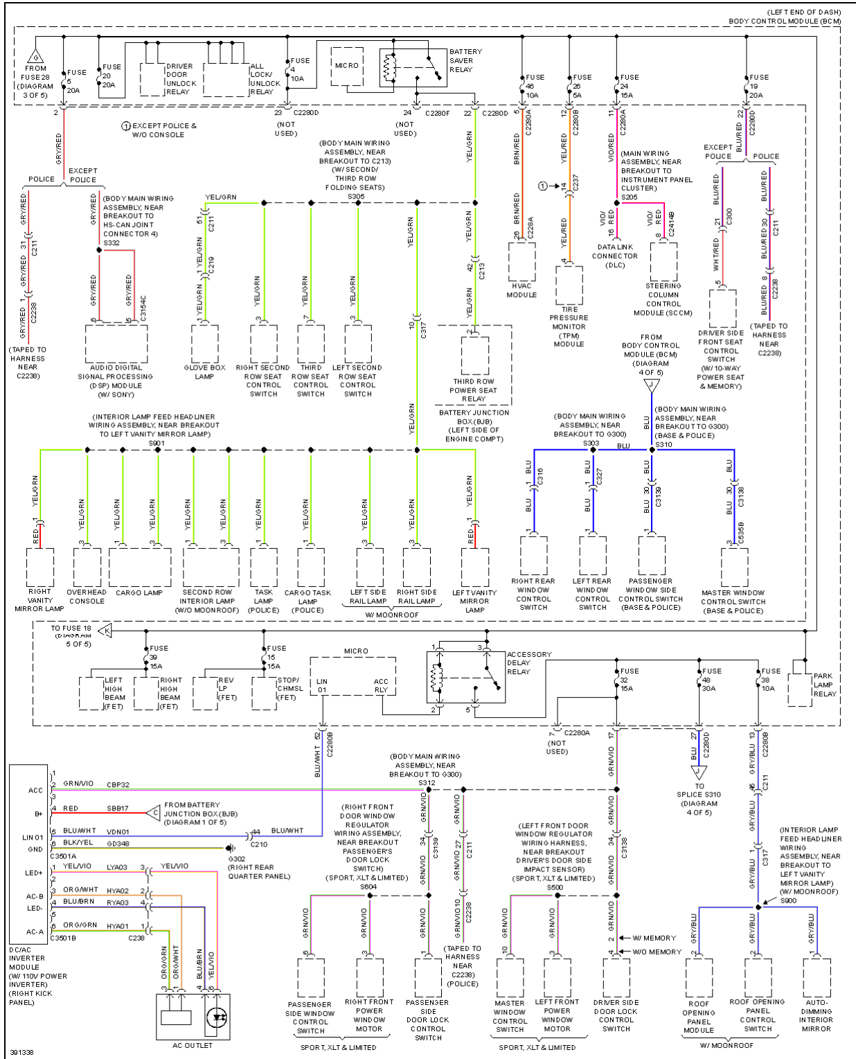
Fig. 80: Power Distribution Circuit (4 of 5)
