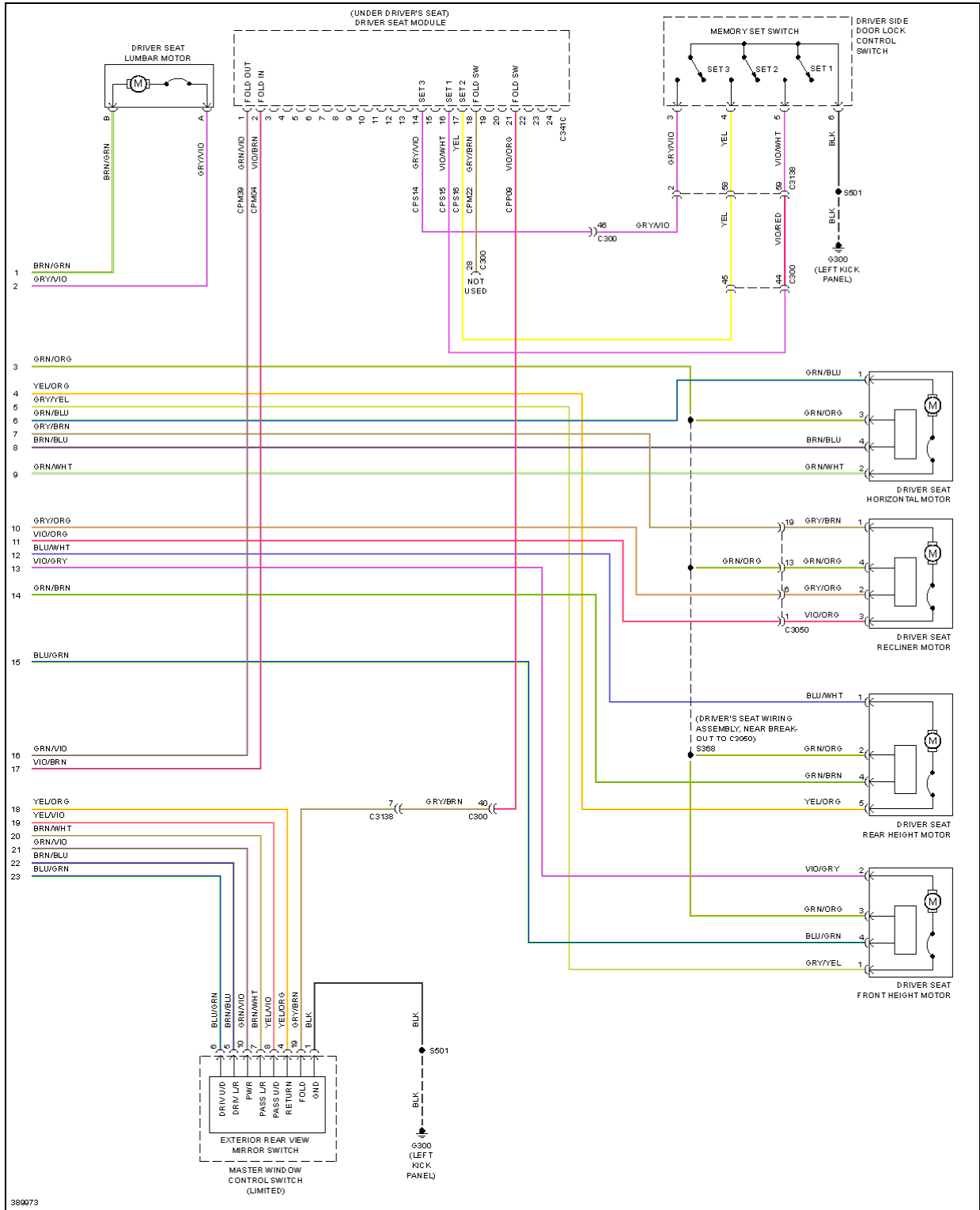
Fig. 69: Memory Seat & Mirrors Circuit (3 of 3)
