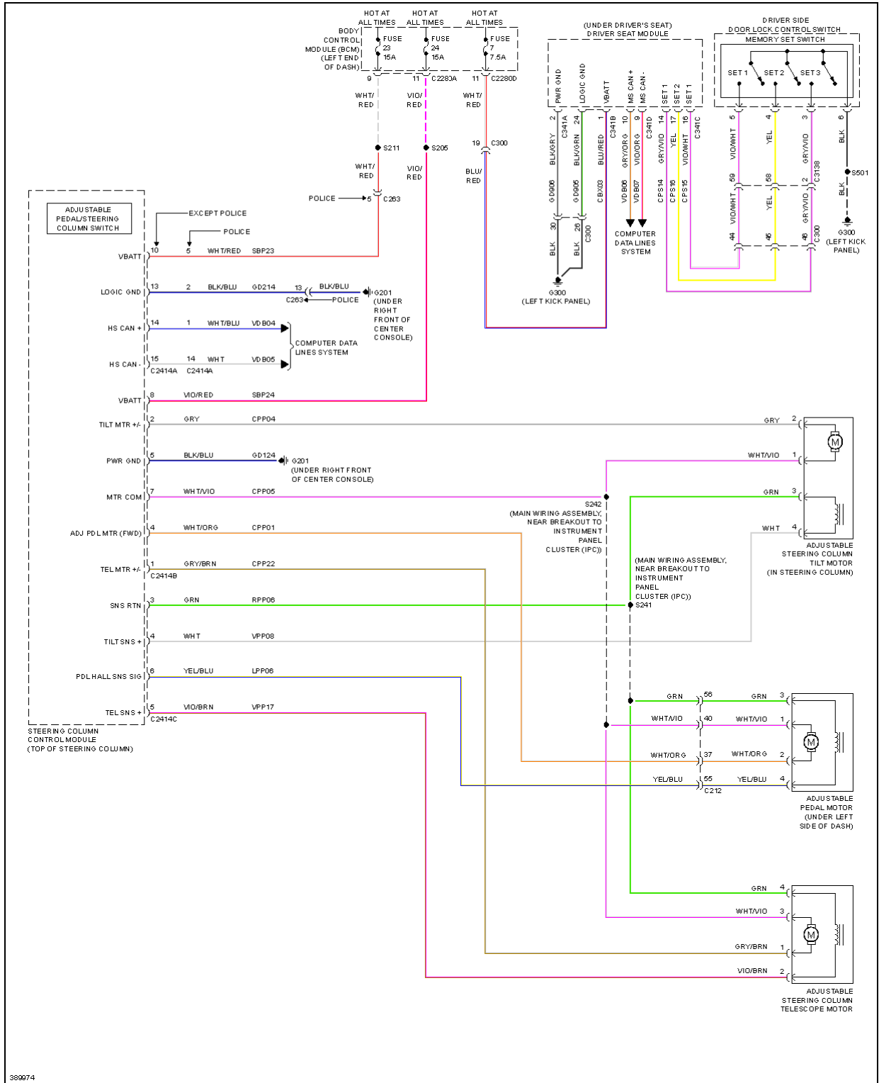
Fig. 66: Adjustable Pedal Circuit
