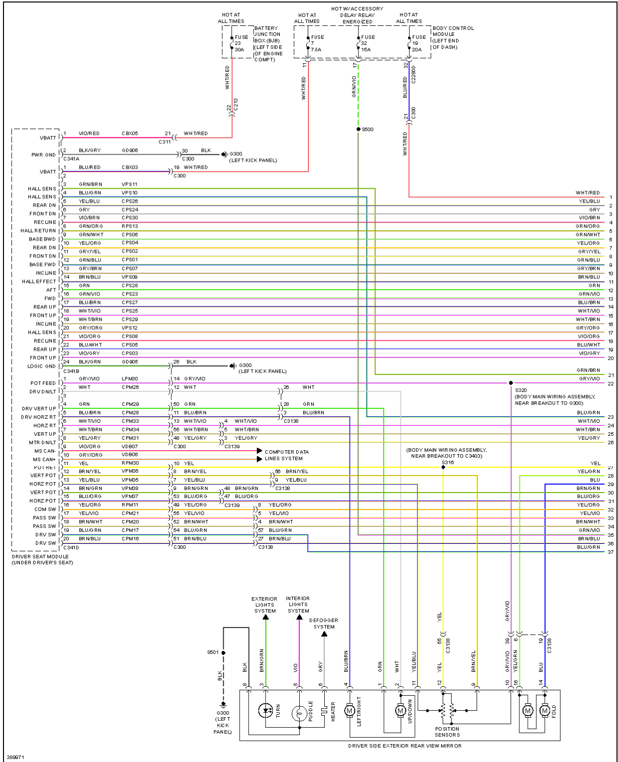
Fig. 67: Memory Seat & Mirrors Circuit (1 of 3)
