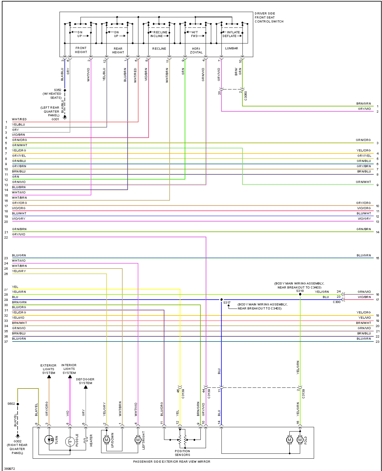
Fig. 68: Memory Seat & Mirrors Circuit (2 of 3)
