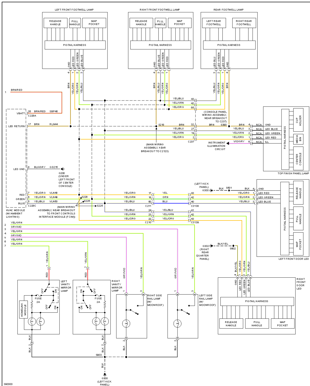
Fig. 64: Courtesy Lamps Circuit (2 of 2)
