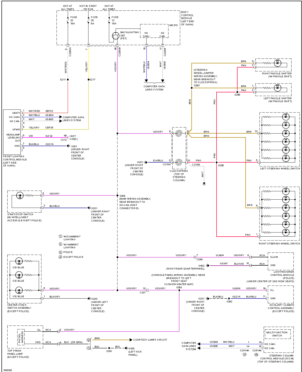
Fig. 65: Instrument Illumination Circuit
