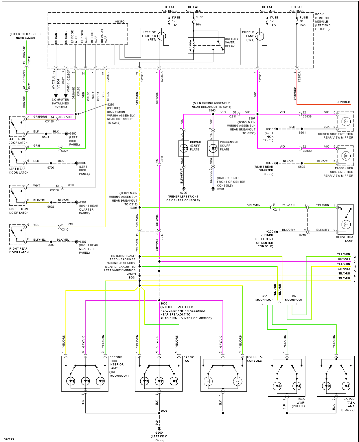
Fig. 63: Courtesy Lamps Circuit (1 of 2)
