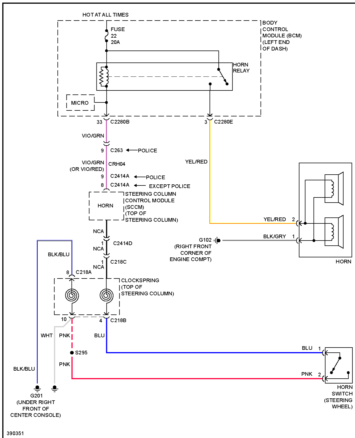
Fig. 61: Horn Circuit
