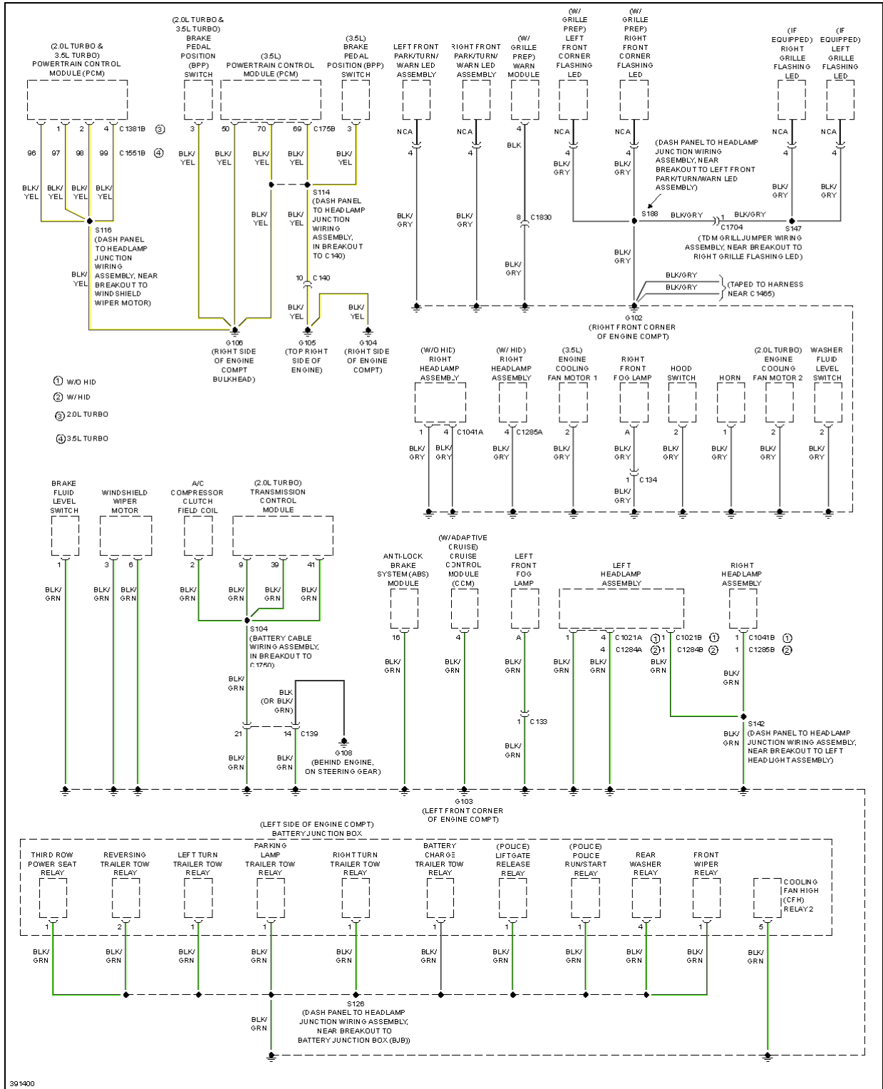
Fig. 53: Ground Distribution Circuit (1 of 6)
