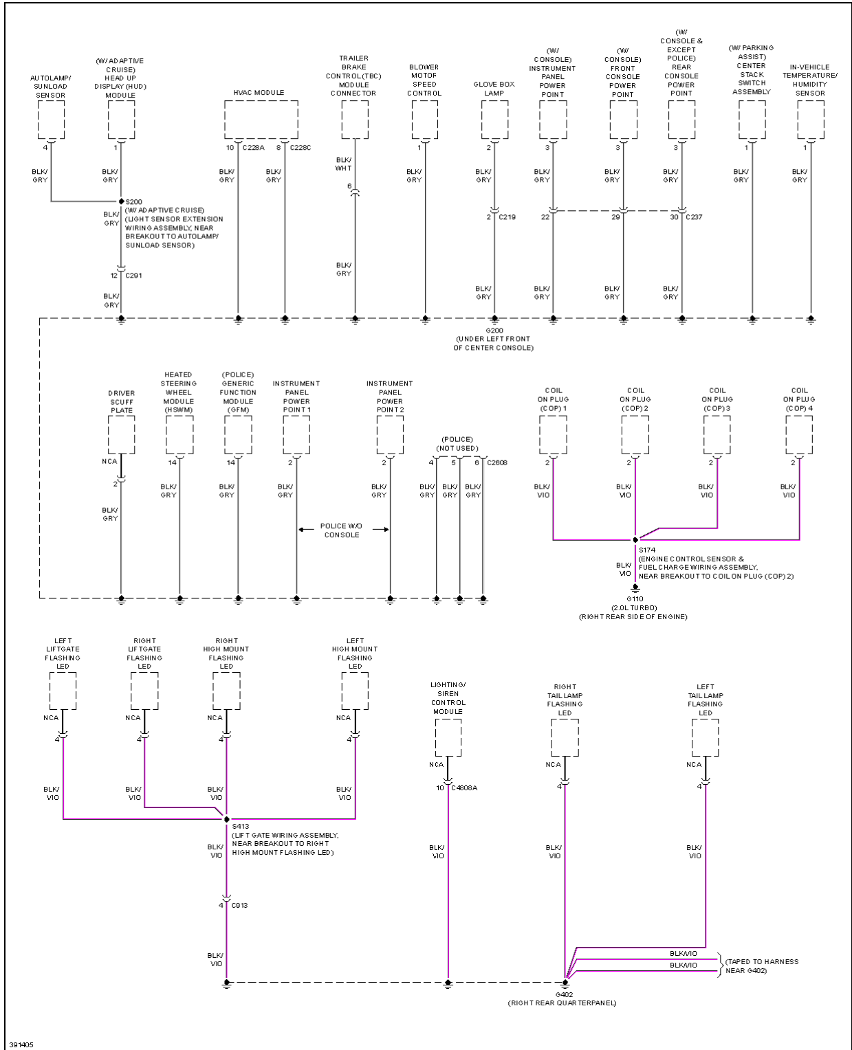
Fig. 58: Ground Distribution Circuit (6 of 6)
