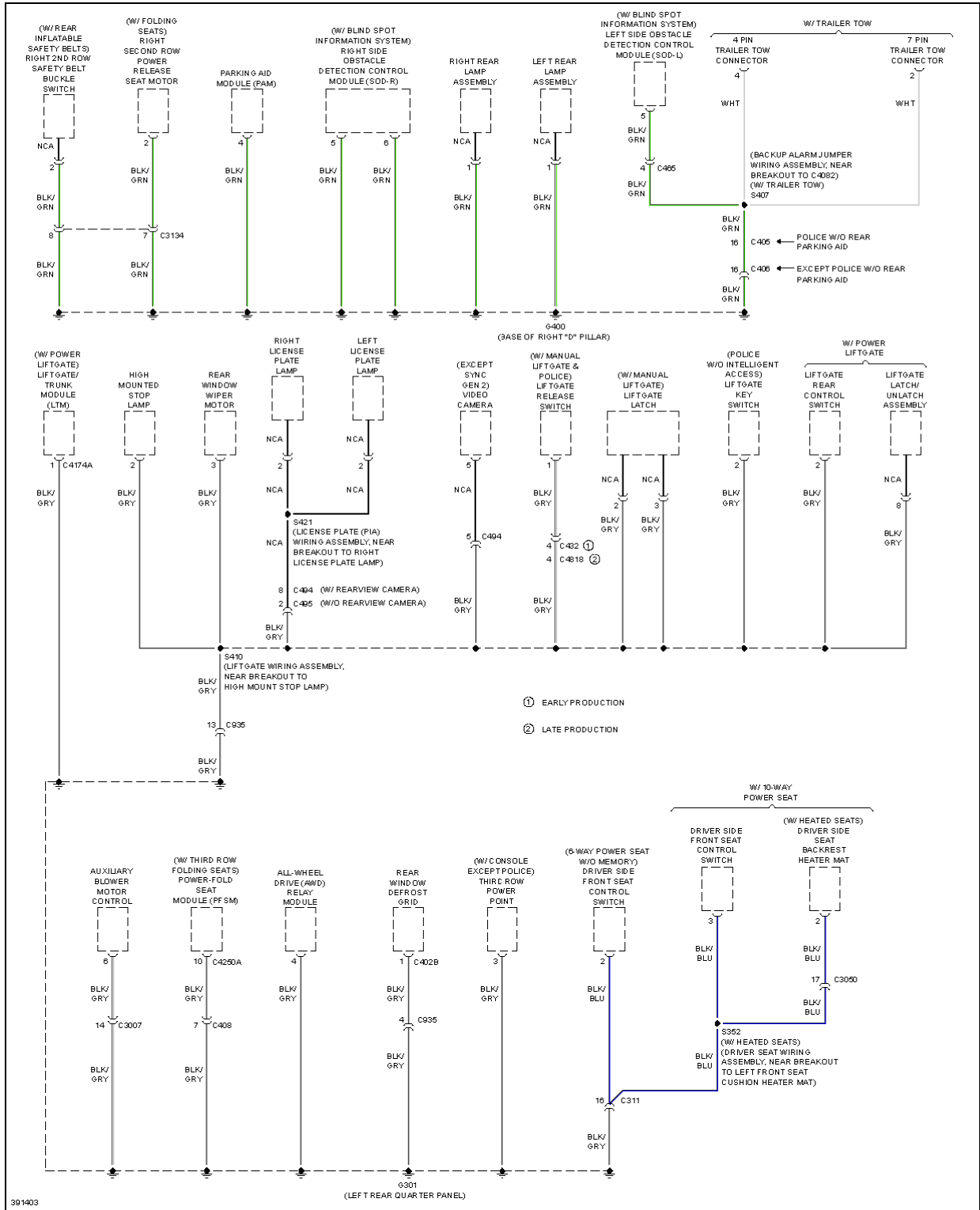
Fig. 56: Ground Distribution Circuit (4 of 6)
