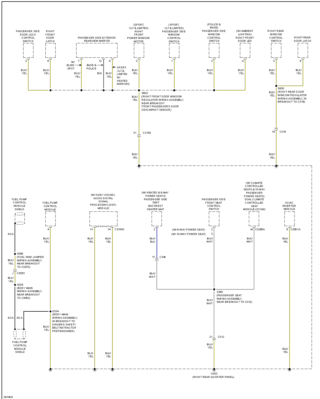
Fig. 57: Ground Distribution Circuit (5 of 6)
