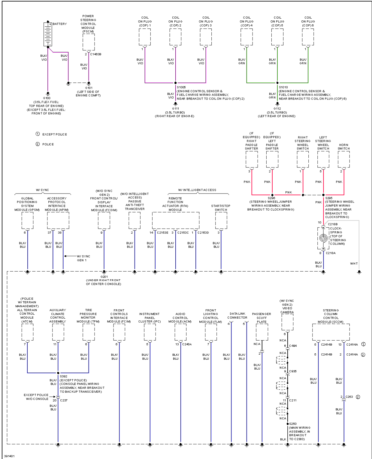
Fig. 54: Ground Distribution Circuit (2 of 6)
