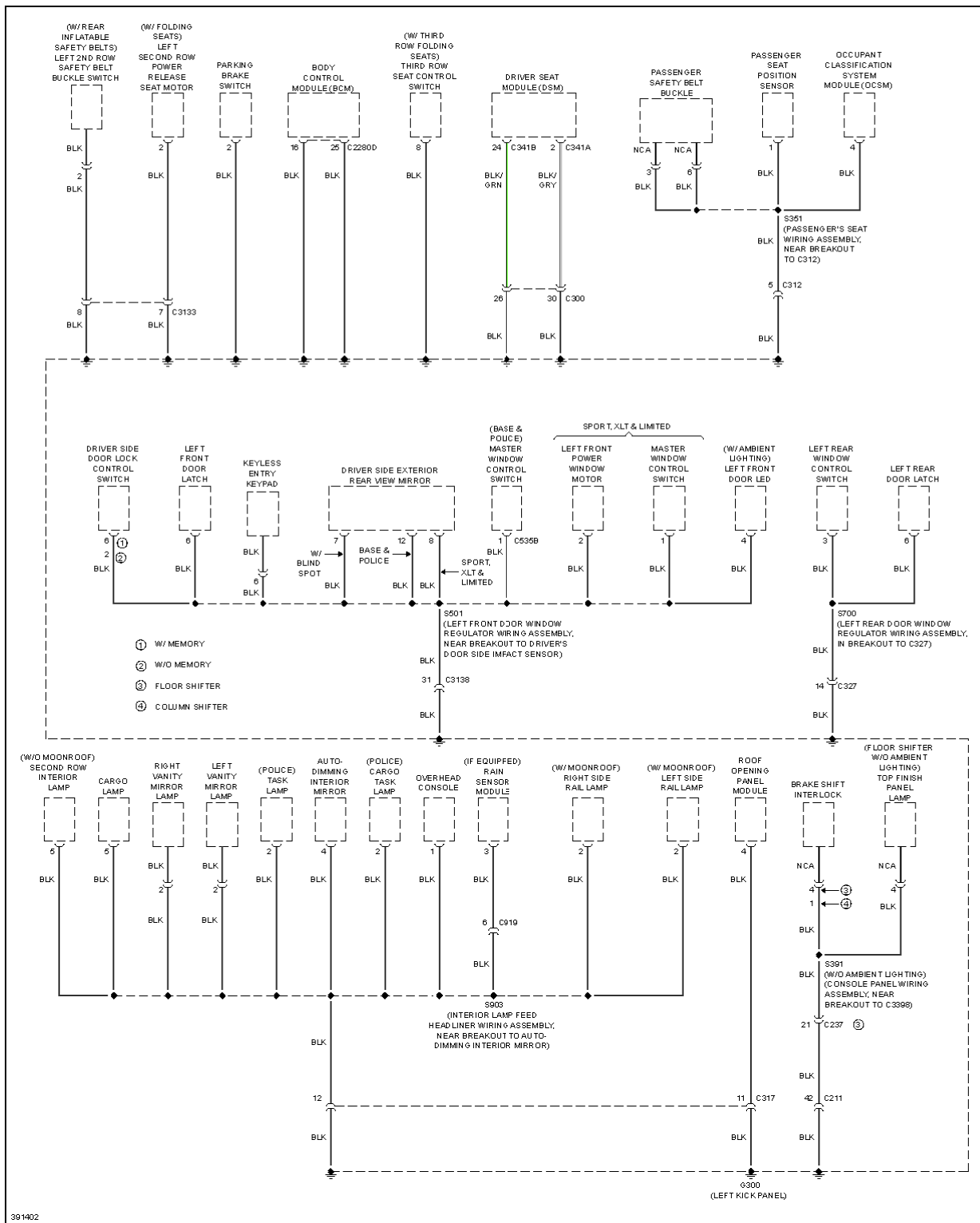
Fig. 55: Ground Distribution Circuit (3 of 6)
