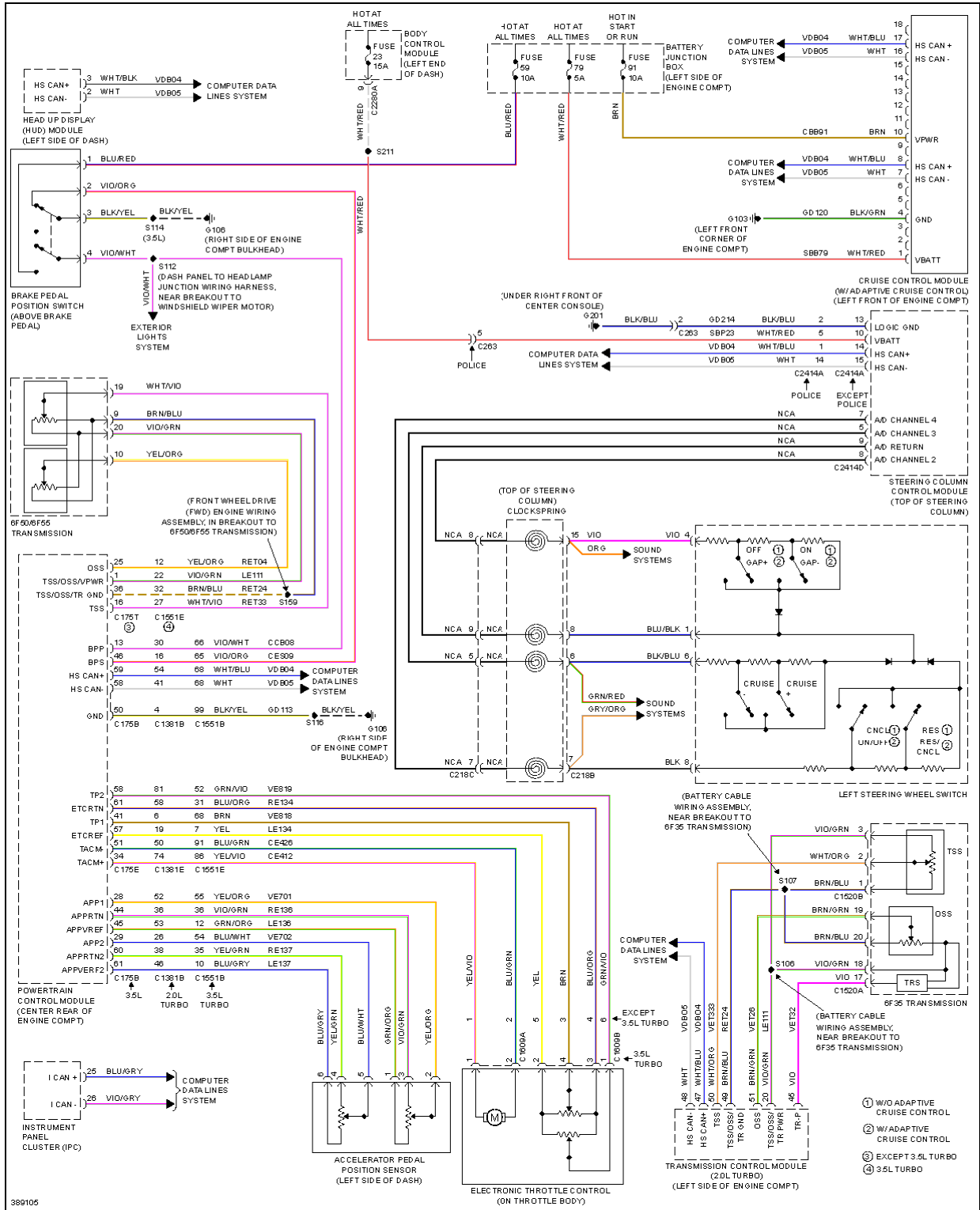
Fig. 23: Cruise Control Circuit
