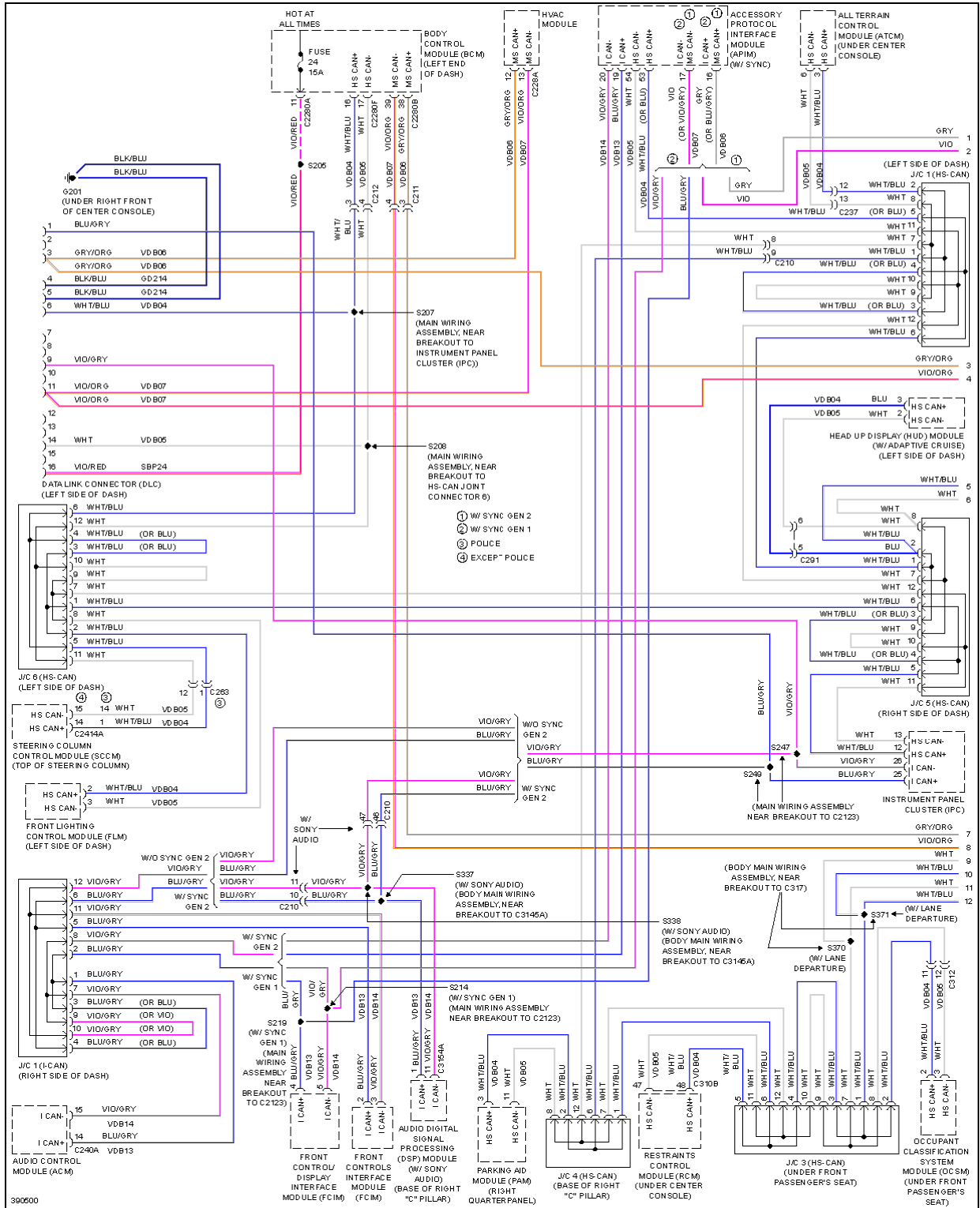
Fig. 20: Computer Data Lines Circuit (1 of 2)
