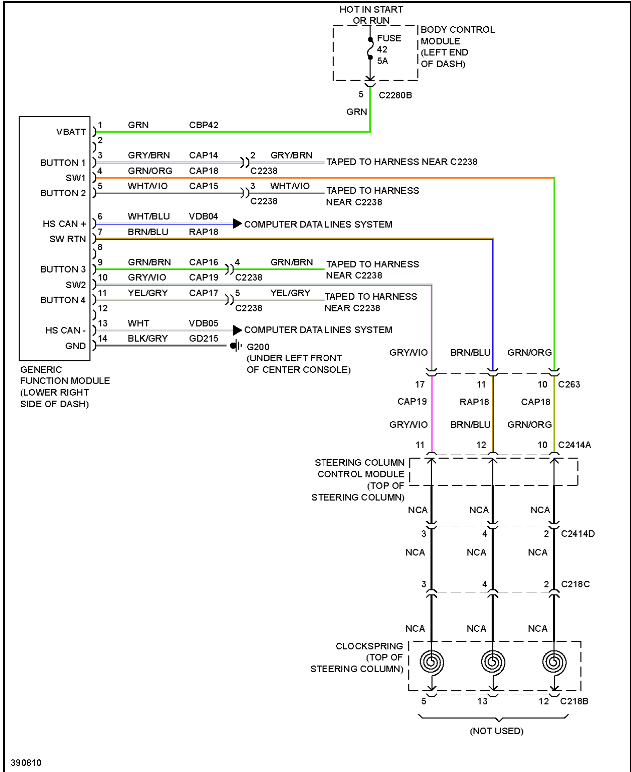
Fig. 19: Generic Electronic Module Circuit
