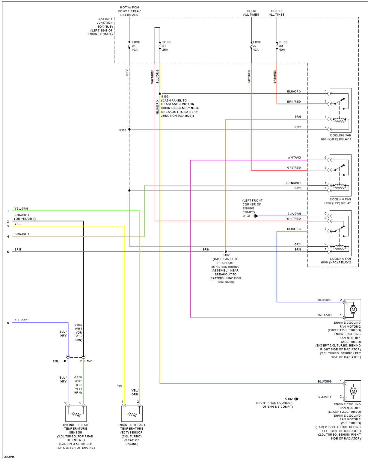
Fig. 9: Manual A/C Circuit (4 of 4)
